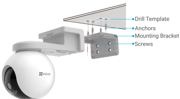
Fig. 1 Ceiling Mount
