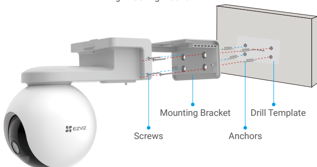
Fig. 2 Wall Mount
